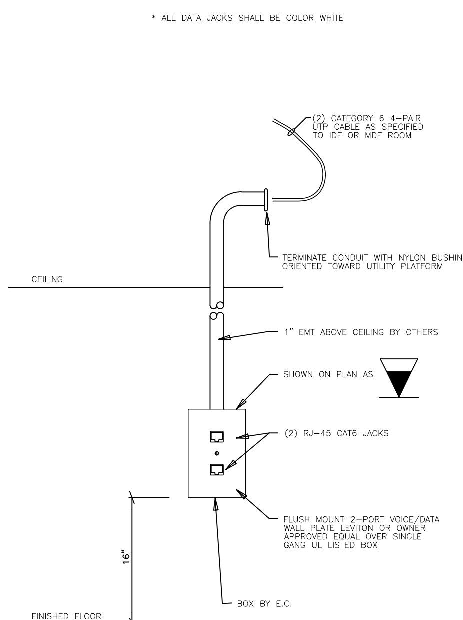
001.2 DUAL DATA OUTLET DETAIL SCALE: NONE
