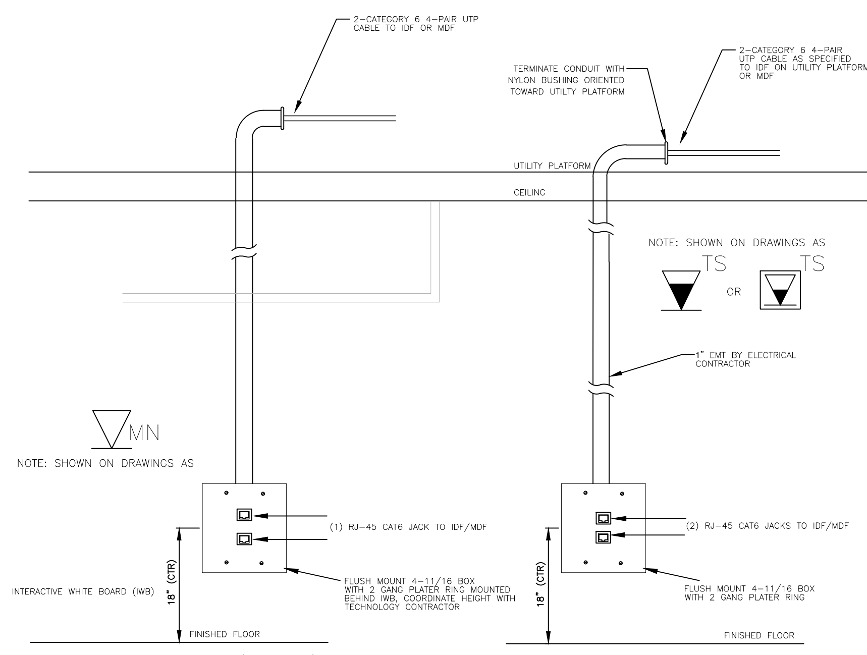
001.3 TEACHERS STATION/IWB OUTLET DETAILS SCALE: NONE
