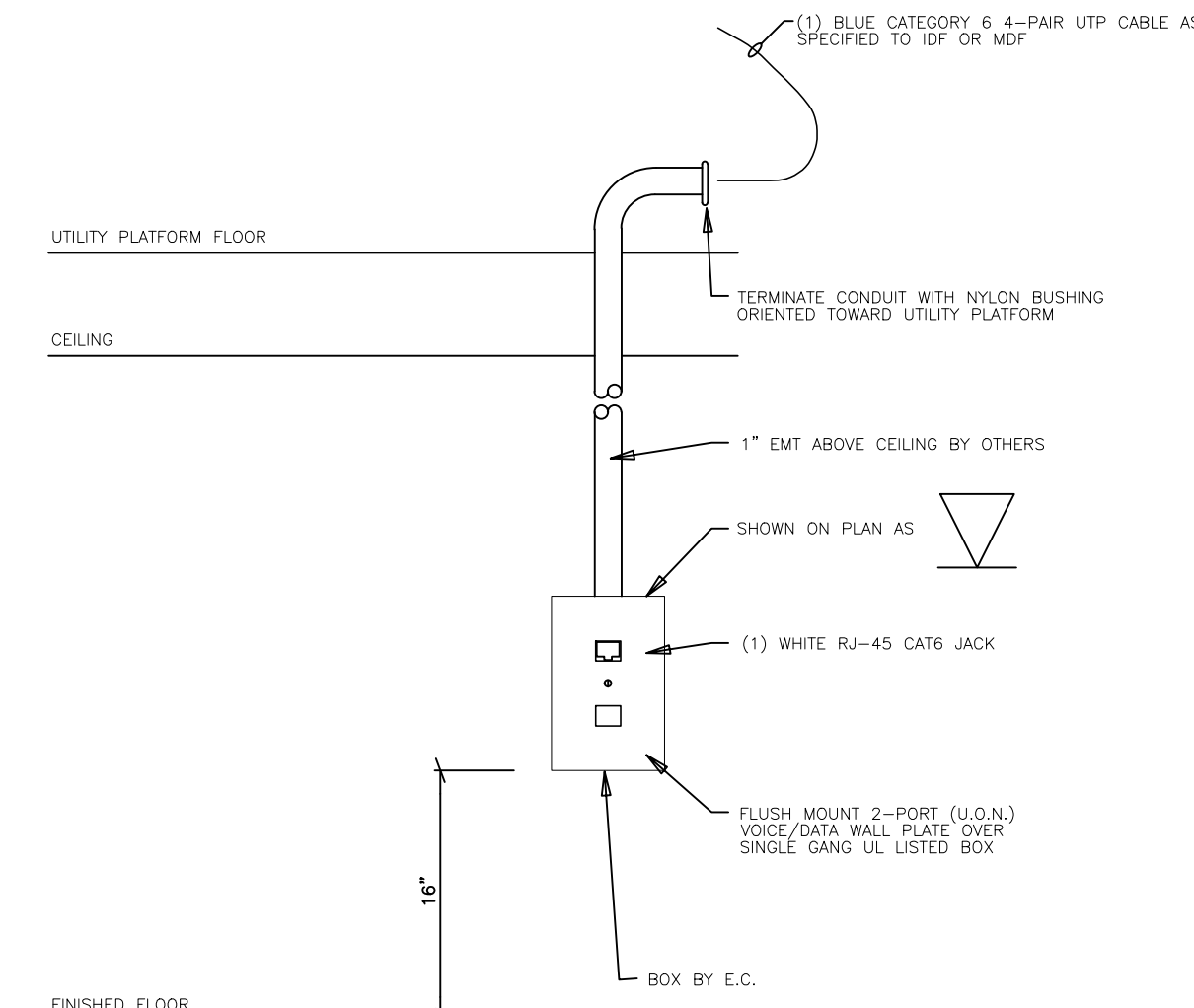
001.6 SINGLE DATA OUTLET DETAIL SCALE: NONE
