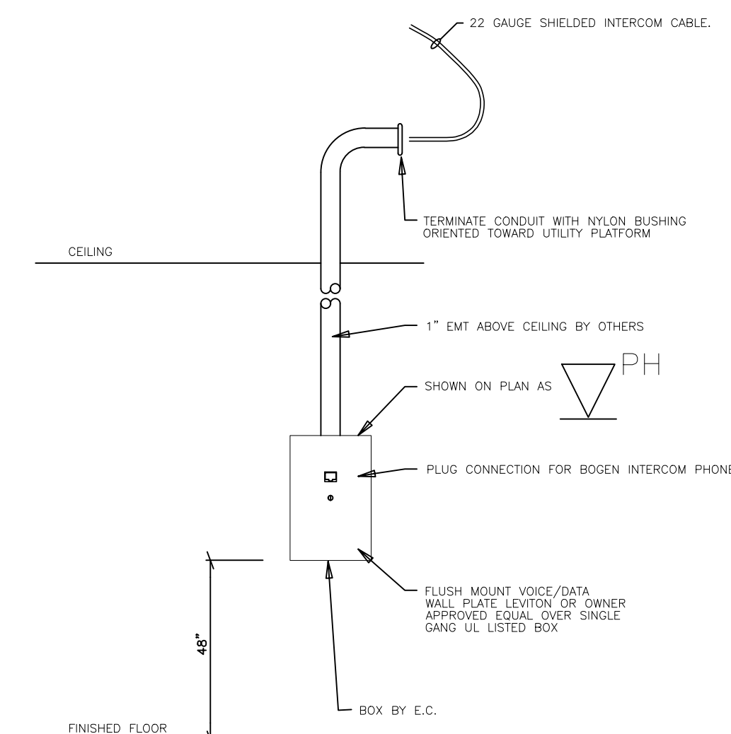
001.4 INTERCOM PHONE DETAIL SCALE: NONE
