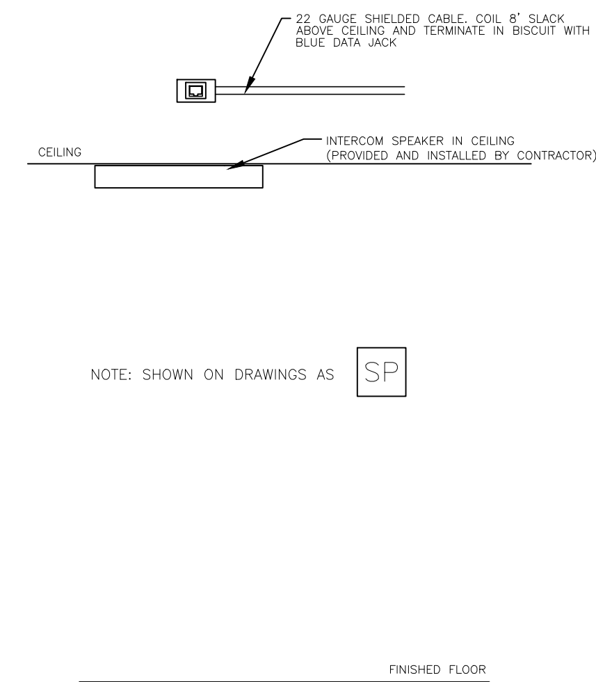
001.1 SPEAKER OUTLET DETAIL SCALE: NONE
