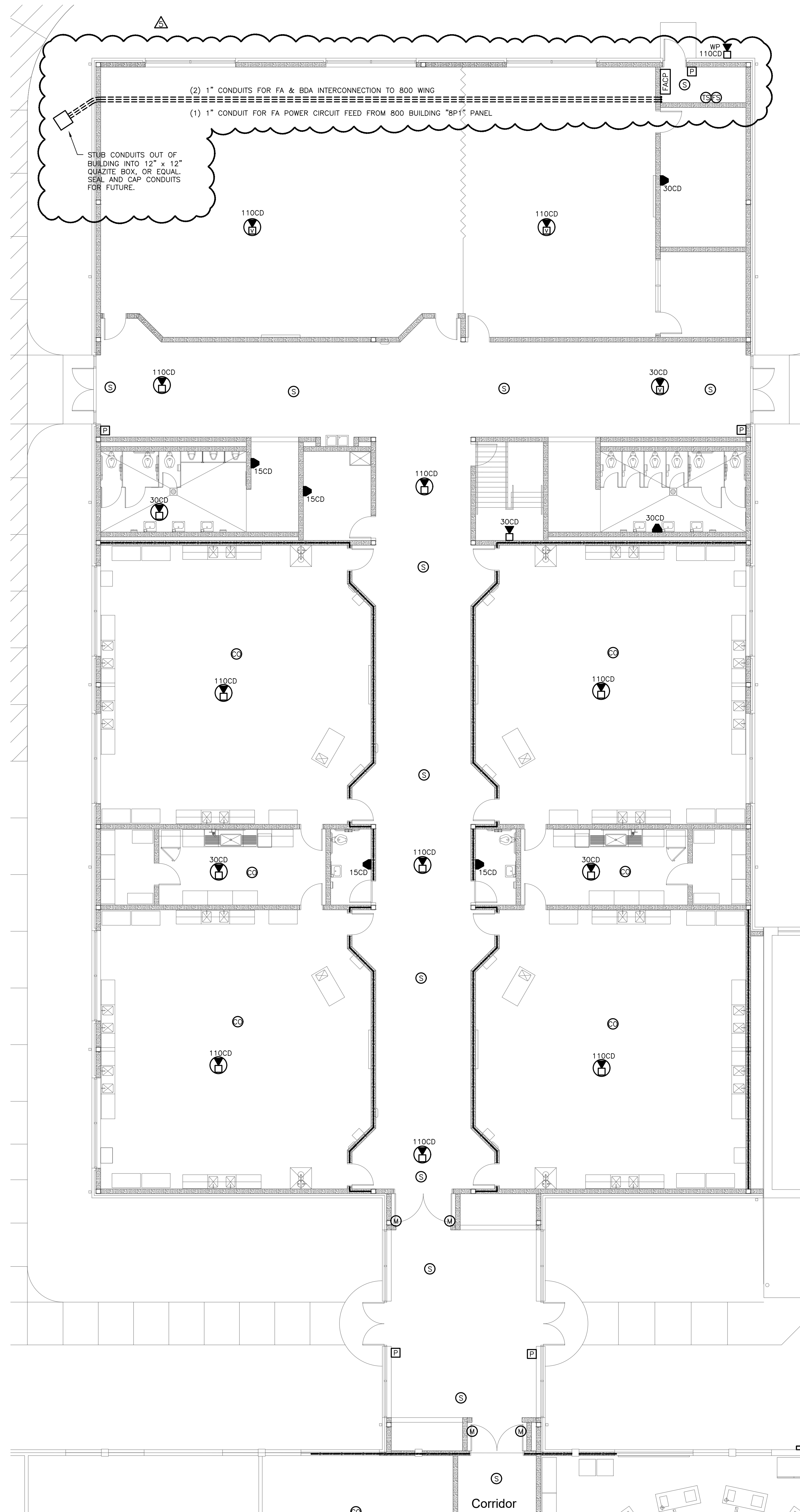
501.2 BASE BID - SCIENCE WING FIRE ALARM PLAN SCALE: 1/8" = 1'-0"
