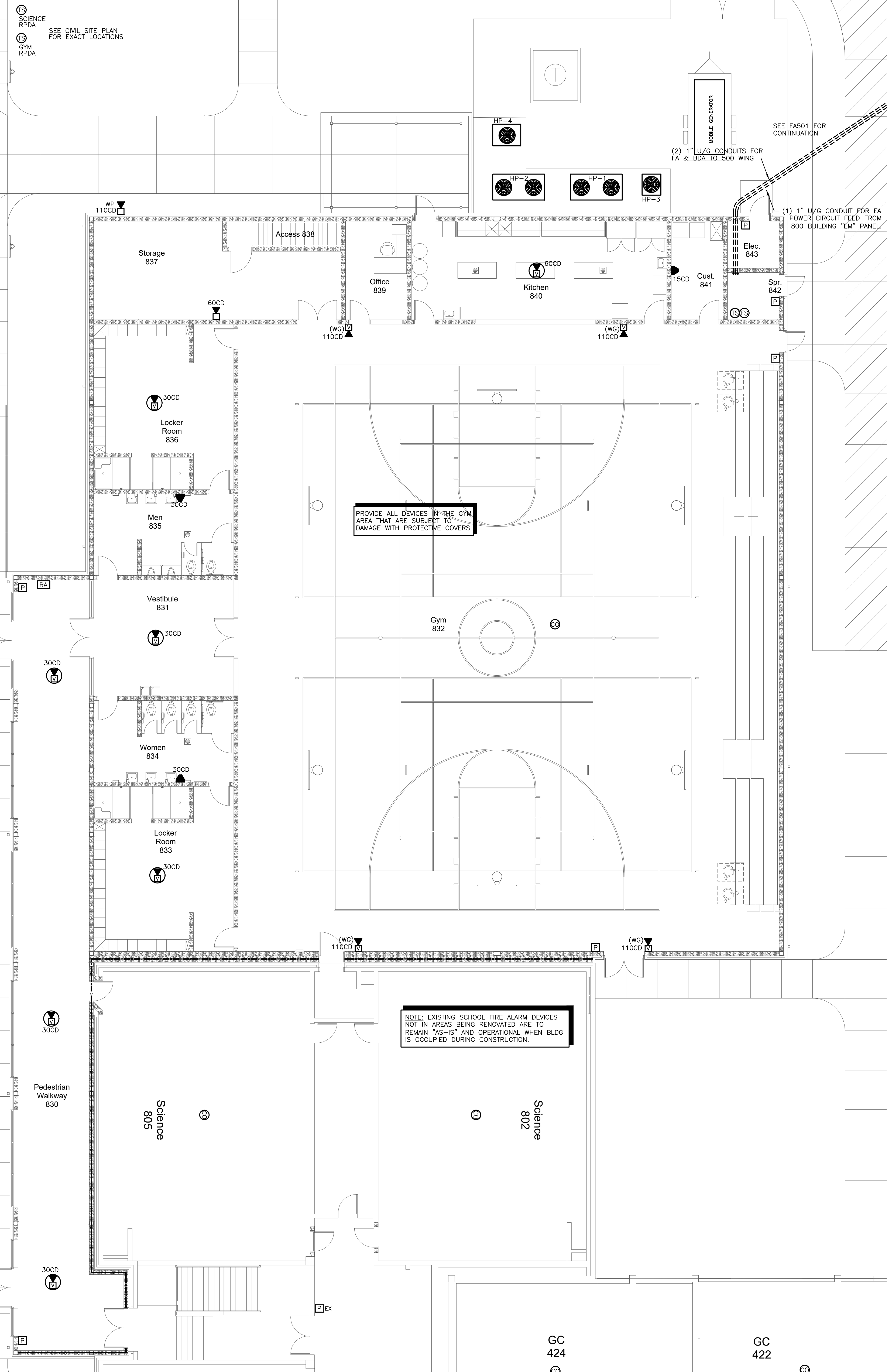
811.2 BASE BID - GYM FIRE ALARM PLAN SCALE: 1/8" = 1'-0"
