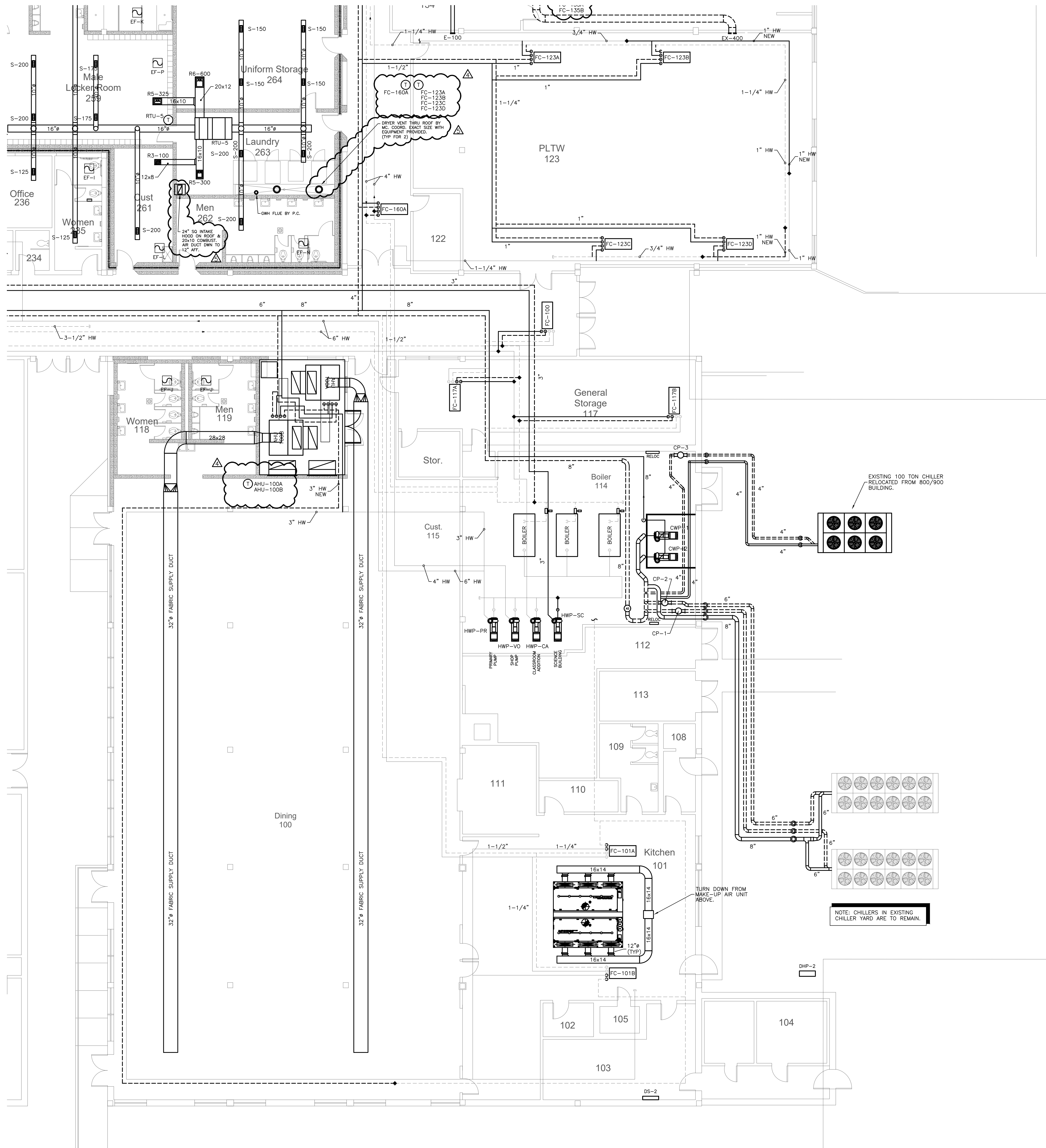
101.1 CAFETERIA AND KITCHEN MECHANICAL PLAN SCALE: 1/8" = 1'-0"
