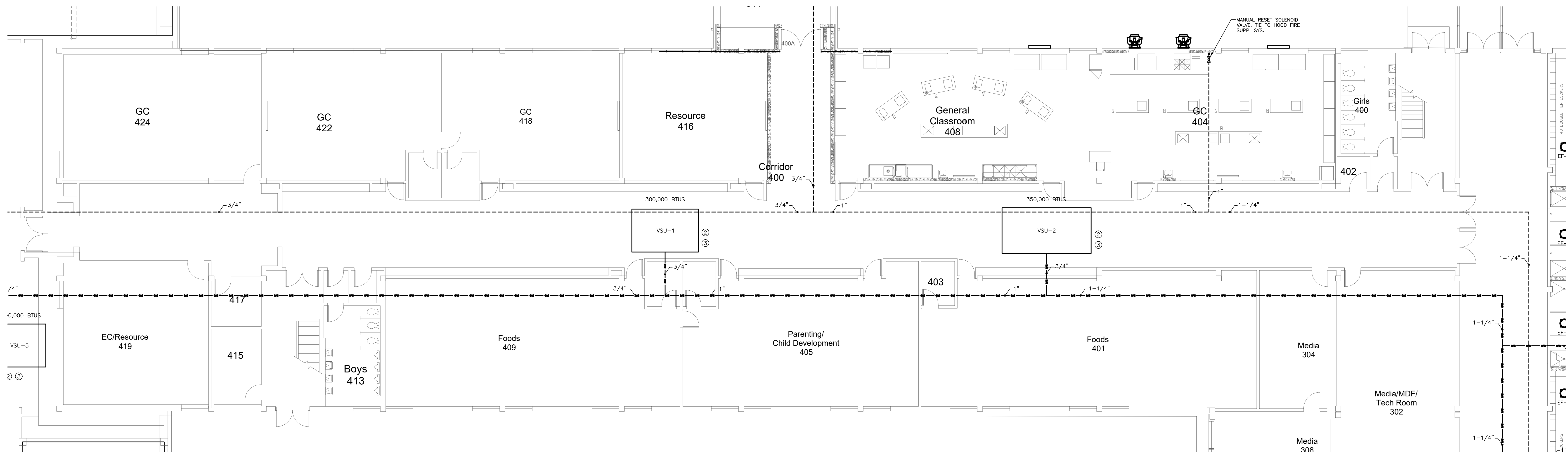
402.1 400 CLASSROOM WING (FIRST FLOOR) GAS & ROOF PLAN SCALE: 1/8" = 1'-0"
