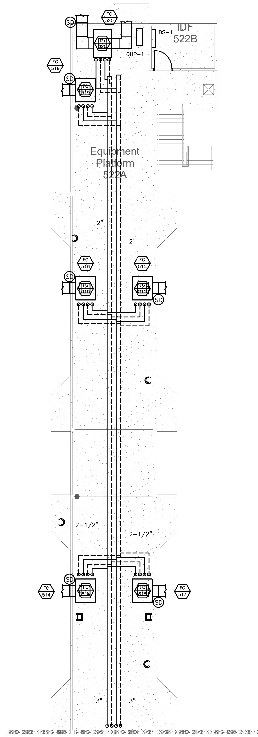
501.2 500 CLASSROOM WING MECHANICAL PIPING PLAN SCALE: 1/8" = 1'-0"
