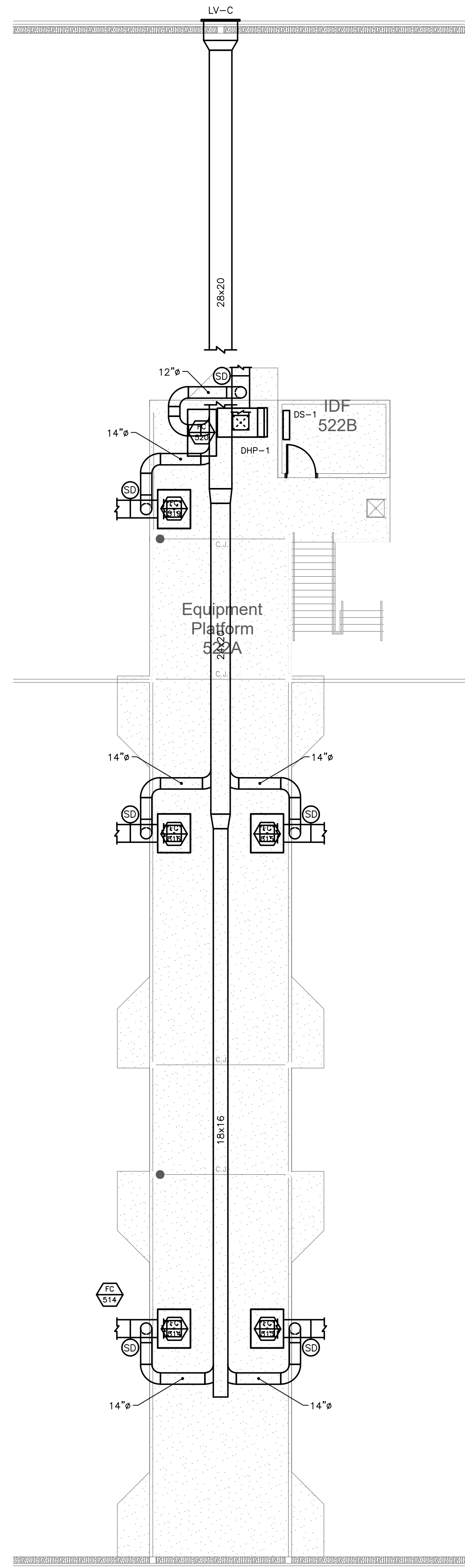
501.2 500 CLASSROOM WING MECHANICAL PLATFORM PLAN SCALE: 1/8" = 1'-0"
